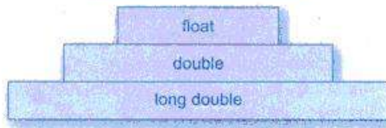
Fig. 2.6 Floating-point types
